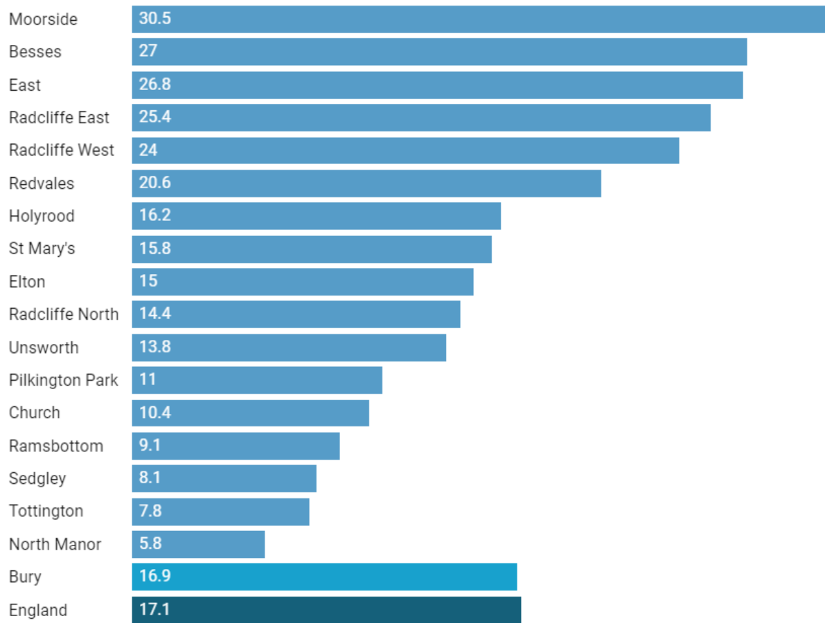
Figure 4: Child Poverty, Income deprivation affecting children index (IDACI), Proportion - %, Wards in Bury, 2019
